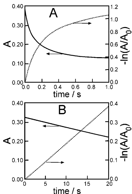
FIGURE 5. Decay of 3 \mu\text{M} \text{dpph}^* in reaction with 0.37 mM curcumin in methanol (A) and in methanol/5 mM acetic acid (B). Reproduced from ref 17. Copyright 2004 American Chemical Society.
